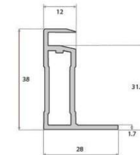
Fig. 10: Frame cross-section and dimensions (mm)
