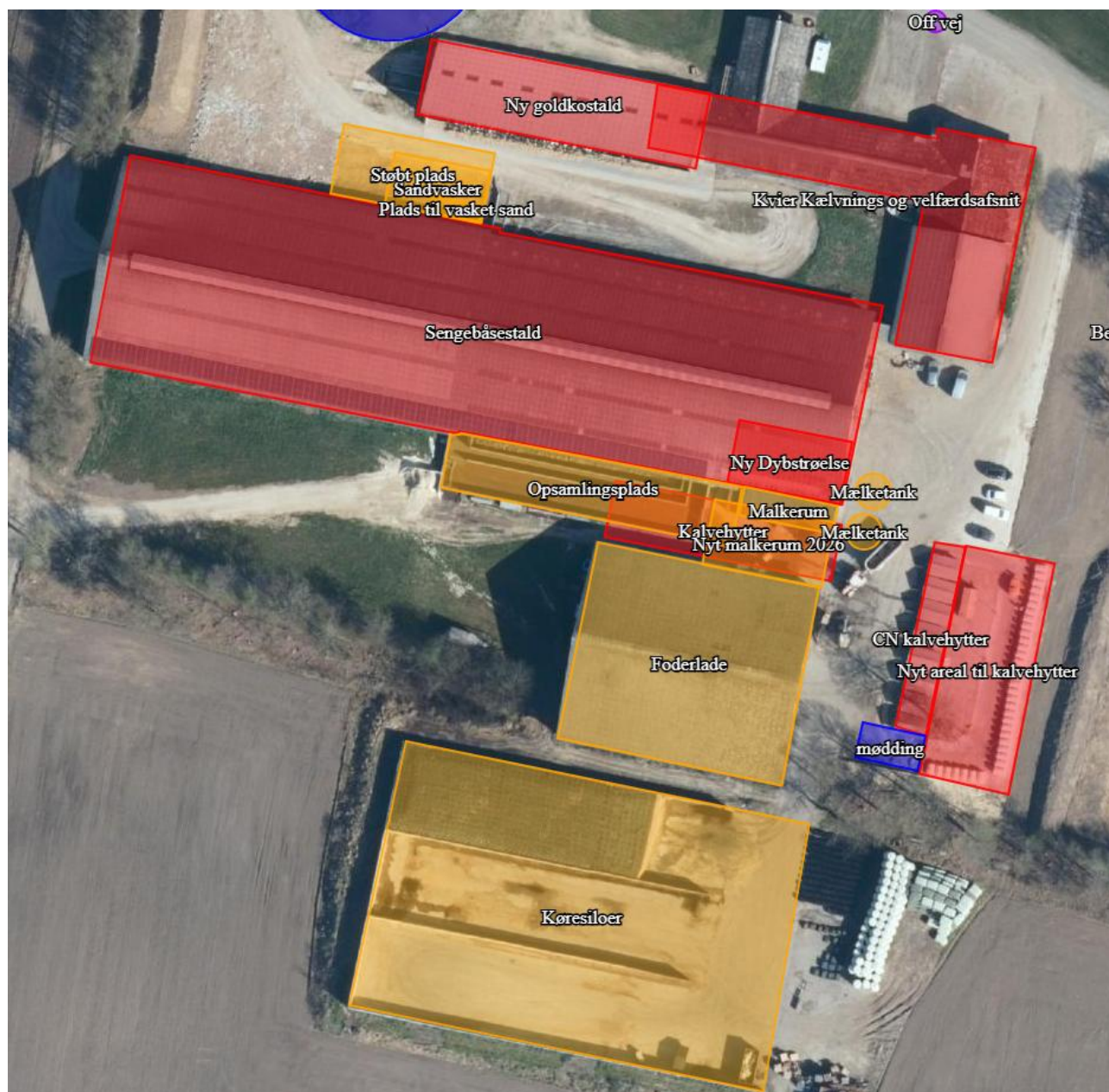
Figur 4. Situationsplan
