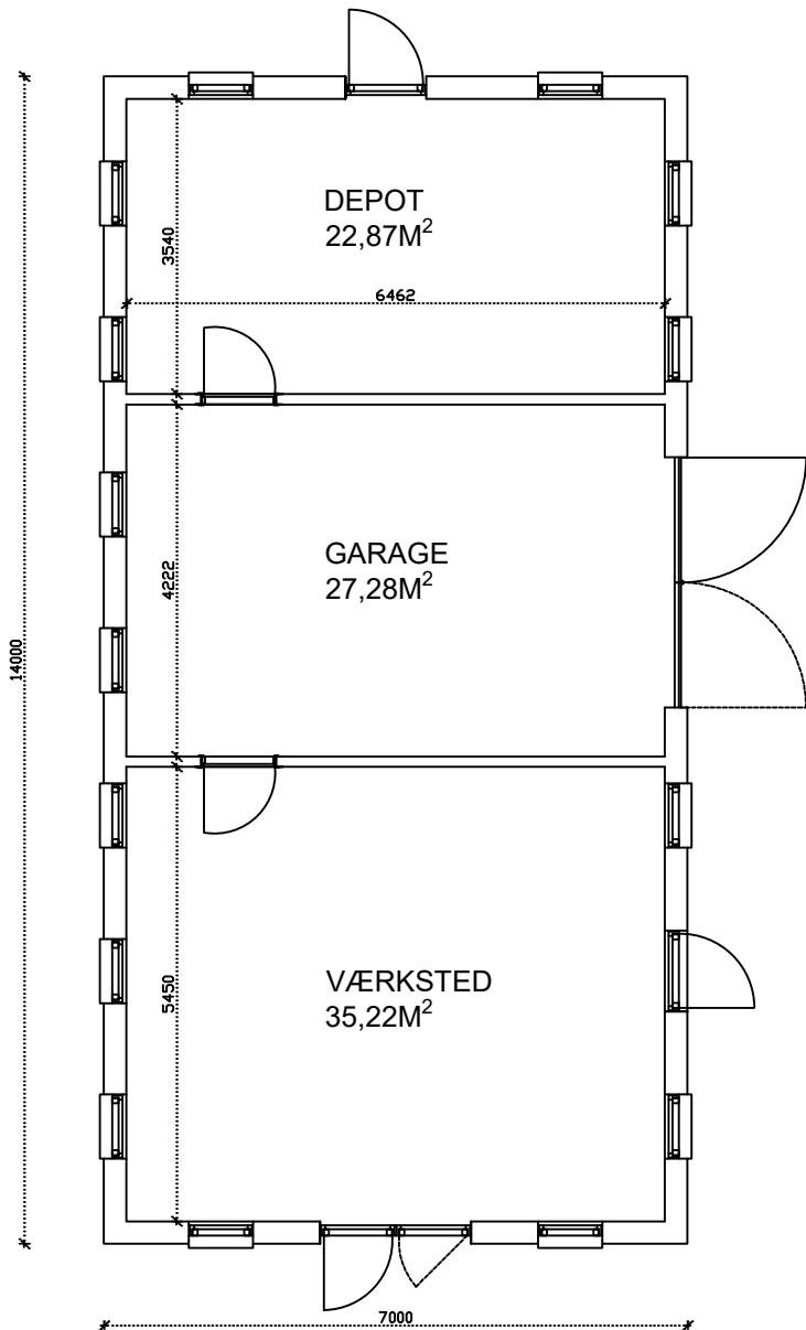
PLAN
