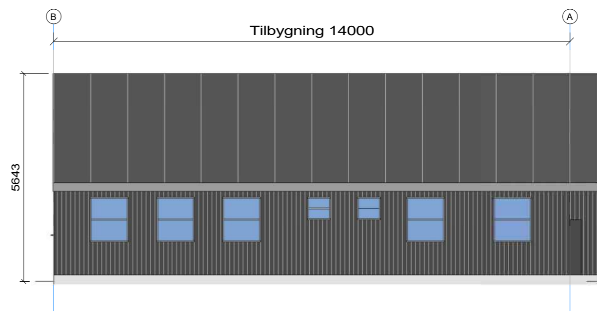
Facade mod vest 1 : 100
